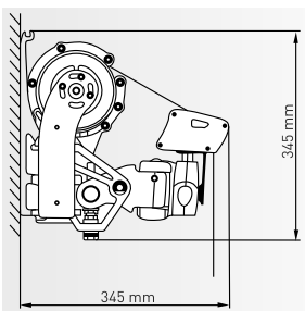
Wandmontage
